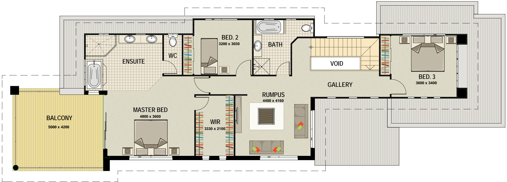
NARROW LOT DESIGN first floor plan
